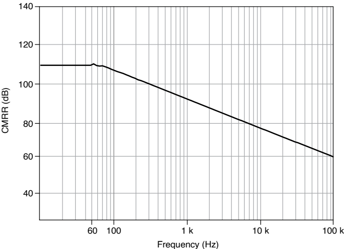
Figure 2. AI CMRR
